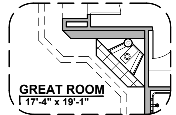
Fireplace Option
