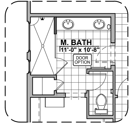
Deluxe Glass Shower Option
