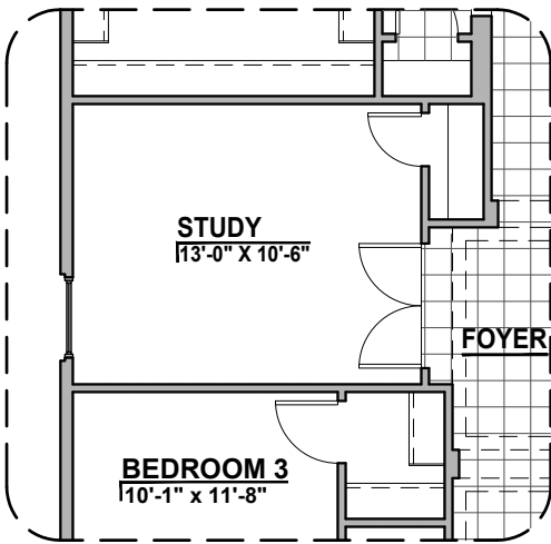
Study Option ILO Flex
