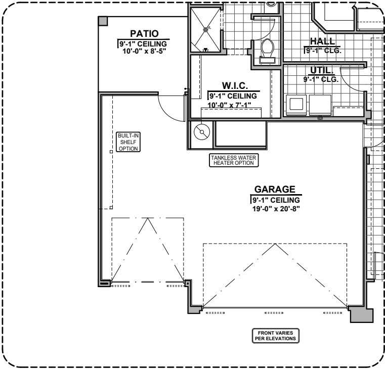
3rd Car Garage
