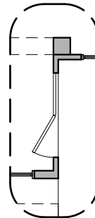
Center Hinge ILO Sliding Glass Door
