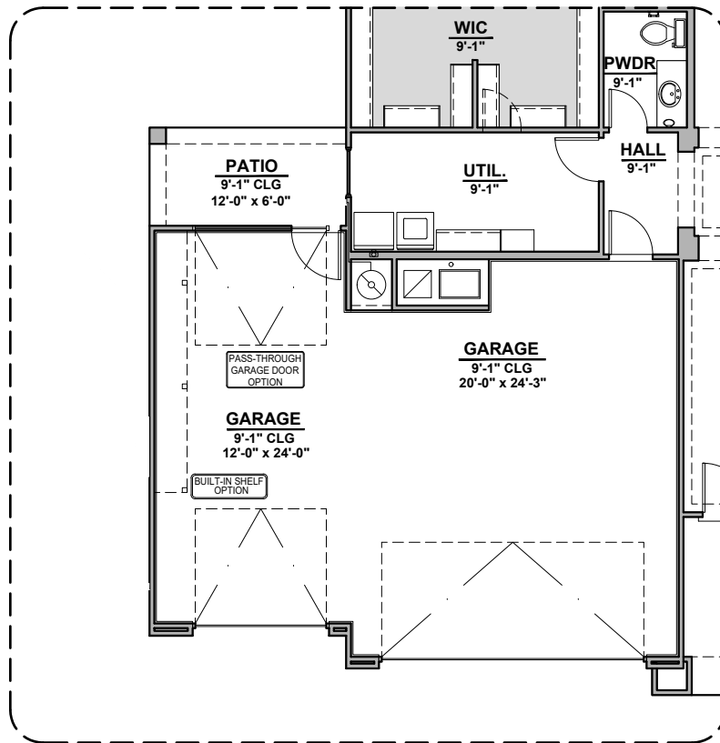
3rd Car Garage
