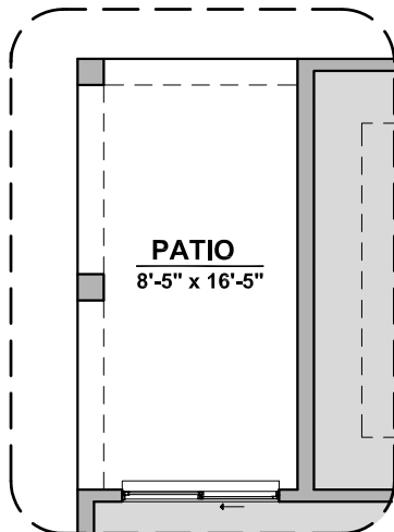
Extended Patio Option
