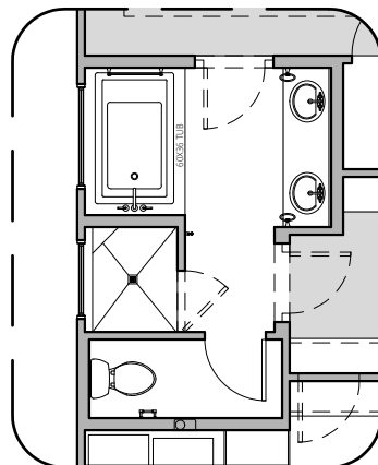
Tub w/ Tile Shower
