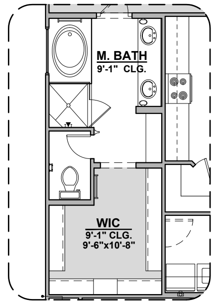
TUB w/ GLASS SHOWER OPTION 1/4" = 1'-0"
