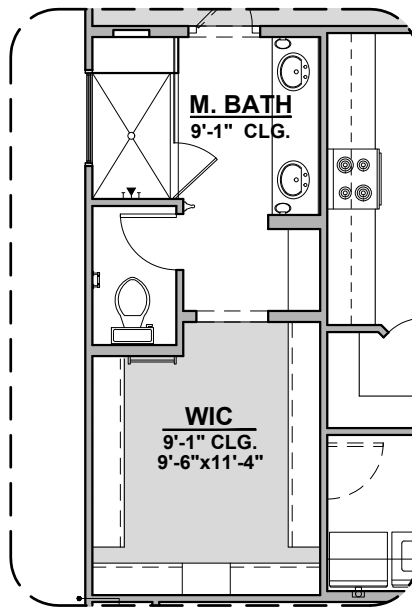
DELUXE GLASS SHOWER OPTION 1/4" = 1'-0"
