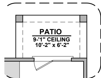
Center Hinge ILO Sliding Glass Door
