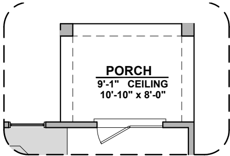
Center Hinge ILO Sliding Glass Door
